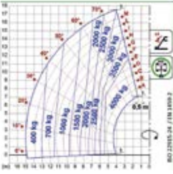
ROTO40.18
