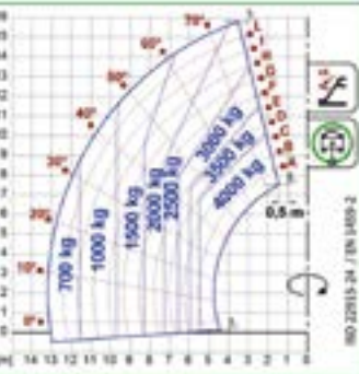
ROTO40.16
